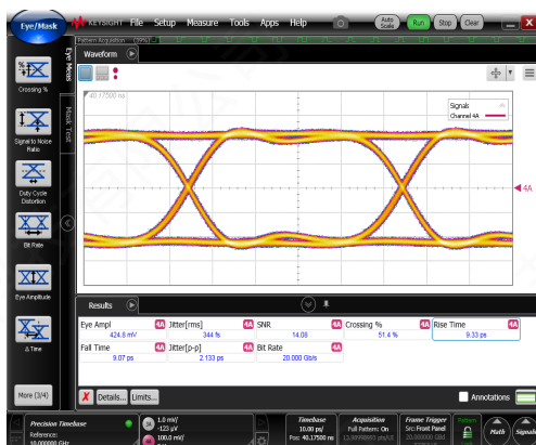
Input signal Eye amplitude = 0.43\text{ V}_{pp}
