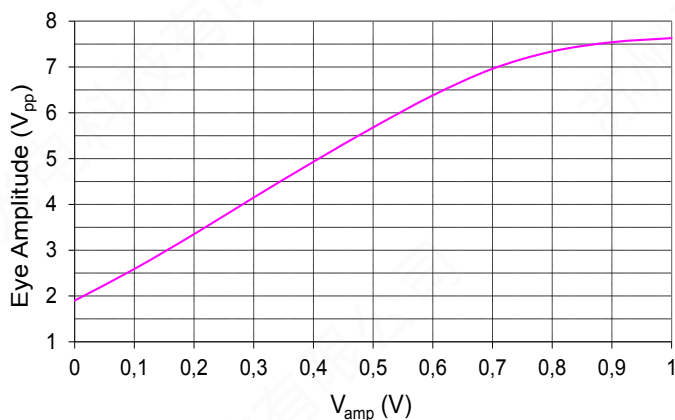
Typical Output Voltage Amplitude vs V_{amp}
